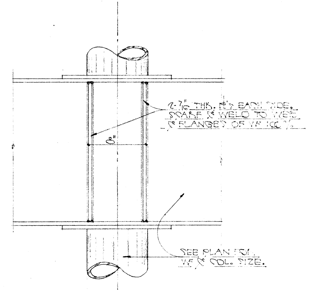
DETAIL 'A' SECTION 3, 4, 5, 6, 7, 8
