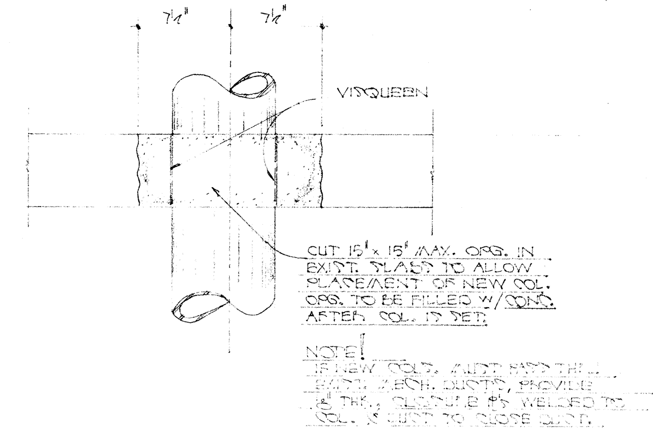
SECTION 1/8" = 1'-0"
